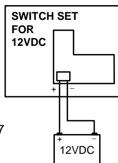
12 Volt Mode Battery Connections
